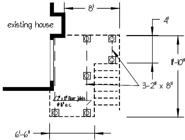
FRAMING PLAN Scale: 1/8" = 1' - 0"
