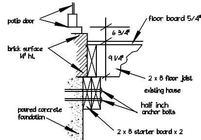
UNDER THE PATIO DOOR DETAIL
